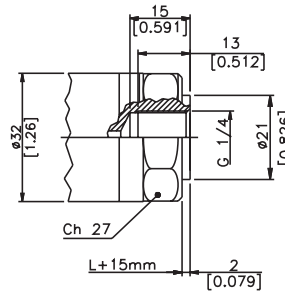
(4) G 1/4 FEMALE
