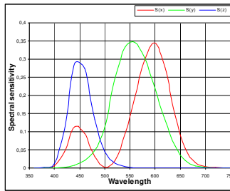
Figure: Spectral sensitivity of True Color sensors
